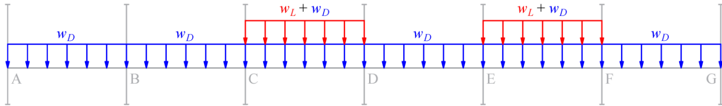
LC3: Span CD and EF are loaded with live load
