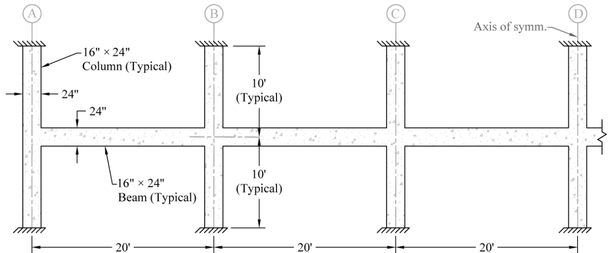
Figure 1 – Continuous Frame Elevation
