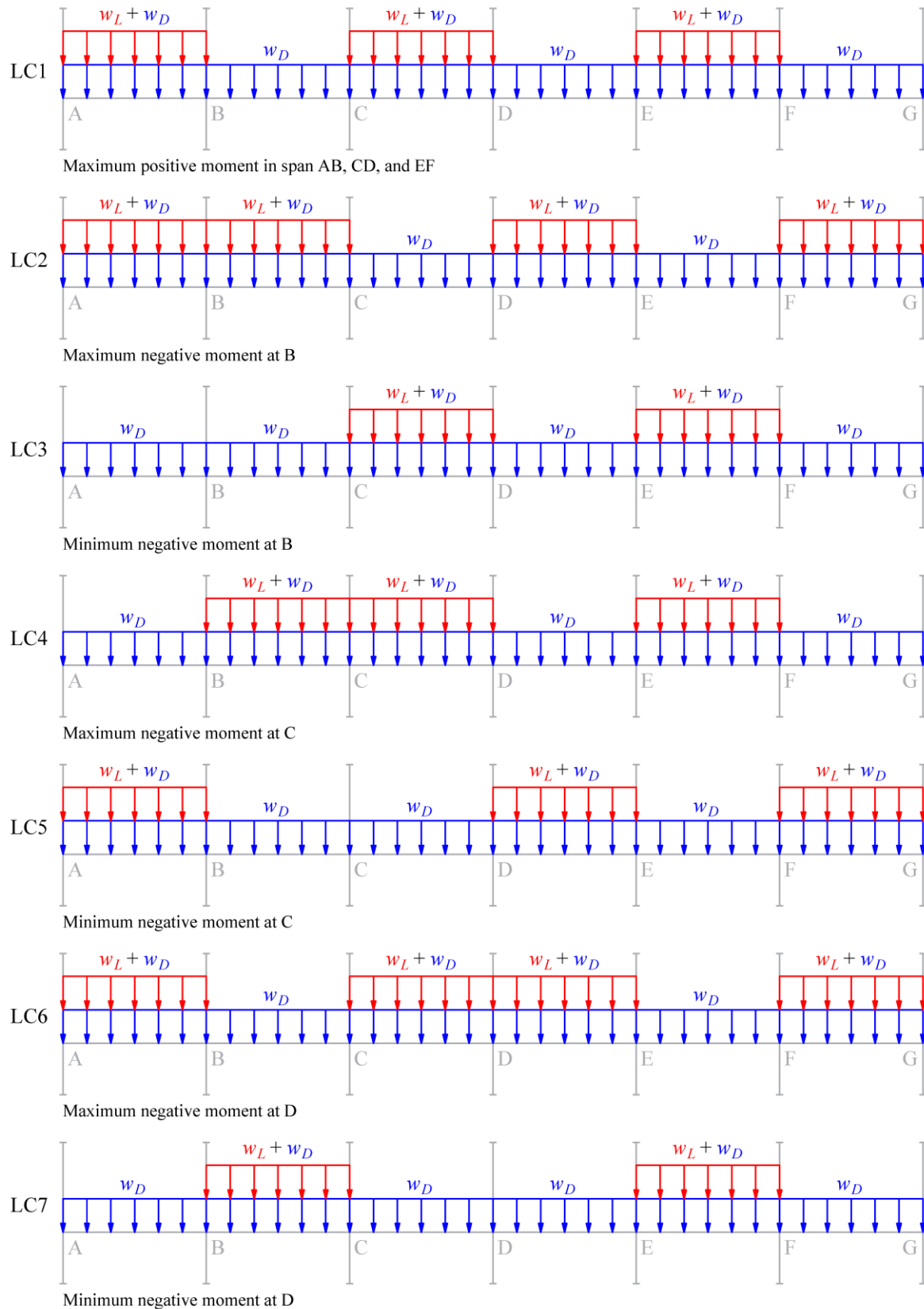
Figure 2 – Loading Scenarios for Six-Span Continuous Frame
